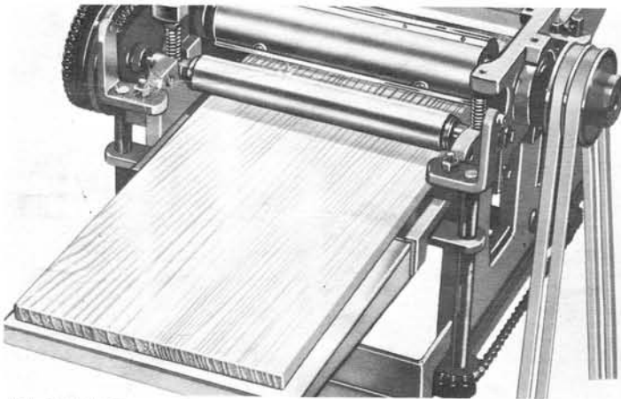
PLANING — Cutterhead uses three planer knives to surface stock up to 12¼-in. wide and up to 6-in. thick. Above photo shows a full 12-in. wide board coming out of the planer surfaced on one side.
