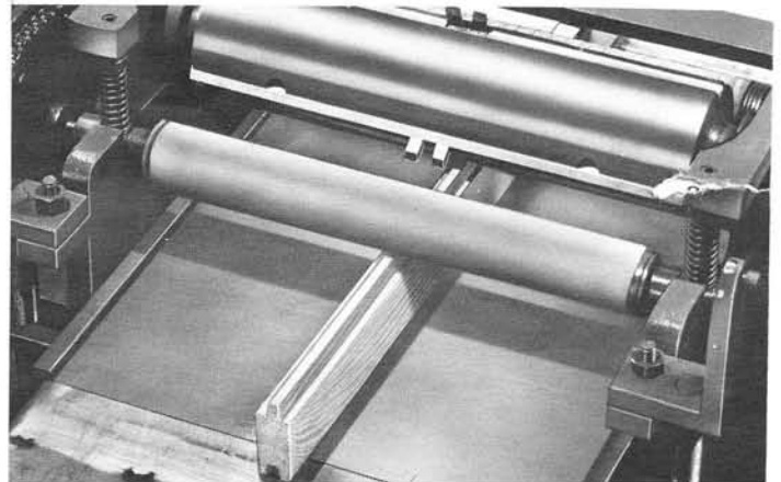
EDGE MOLDING — Tongue-and-Groove Molding is a simple operation on the new planer, one of many molding operations possible by easily and quickly changing the cutters.
