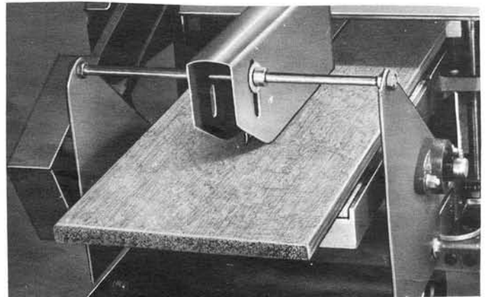
SAWING — Rip stock up to 2¼-inches thick and surface it to desired thickness and pattern in one continuous pass ... all by power feed.
