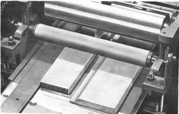
FACE MOLDING — This board is emerging from the new planer, sawed to width, planed to the desired thickness and molded for baseboard use, all with power feed.
